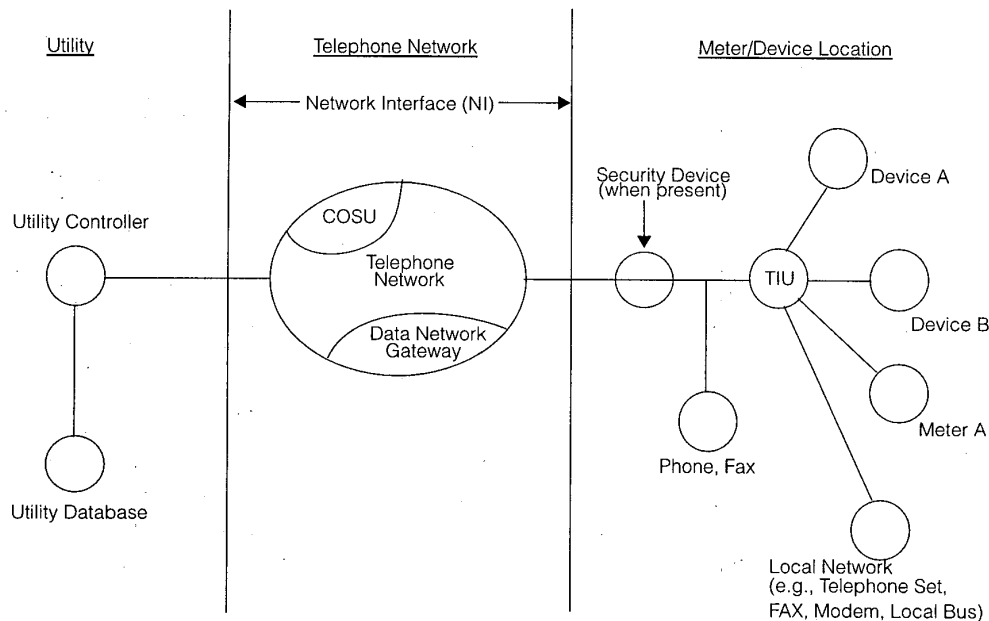
Figure 1—Utility telemetry service architecture for telephone network communications
