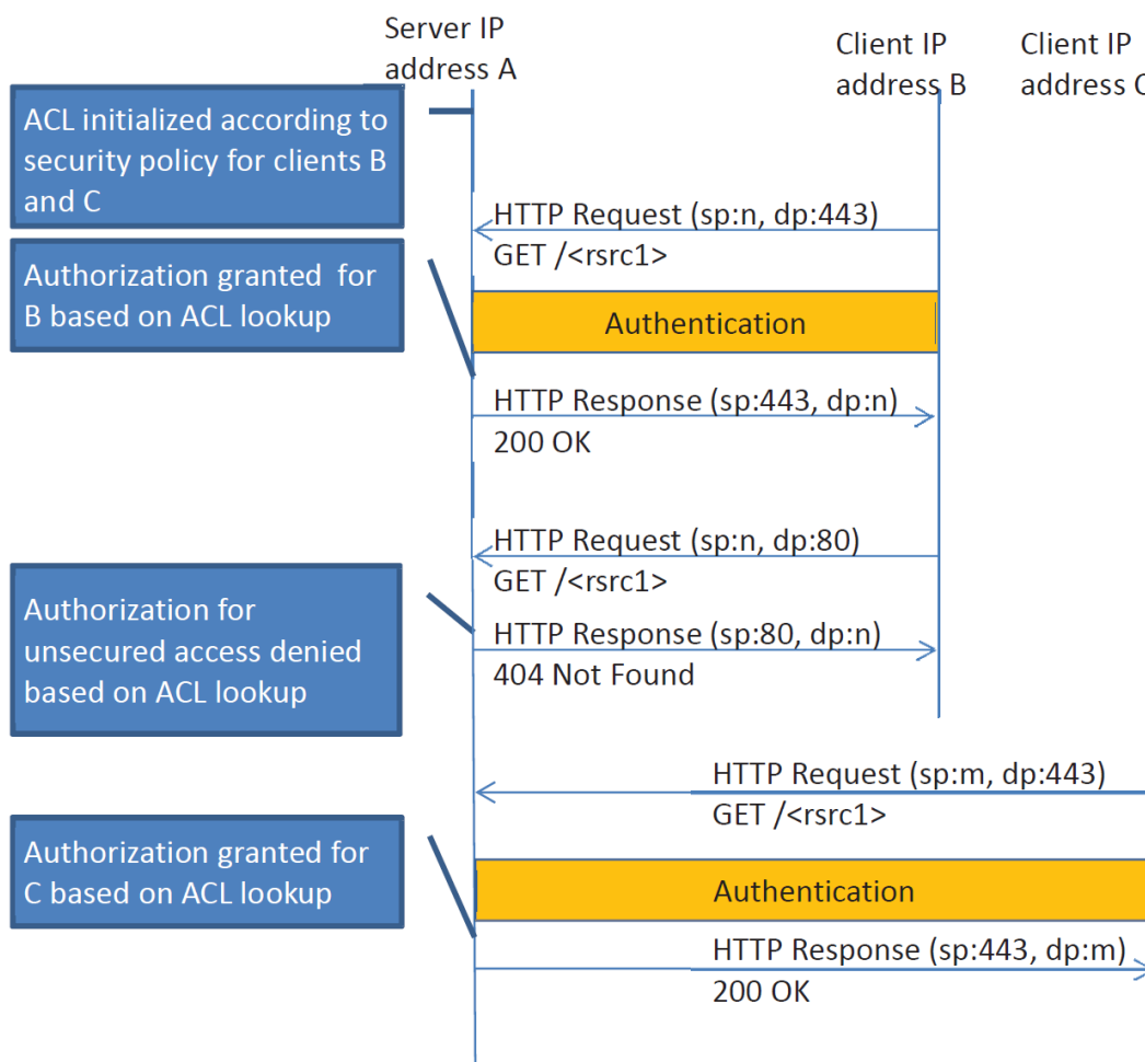
Figure 1—Example device authentication procedure using HTTPS port 443
