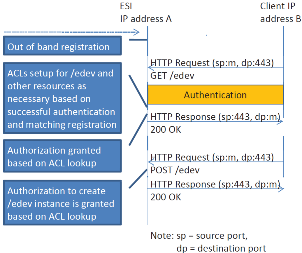
Figure 2—Device authentication with registration procedure examples using HTTPS
