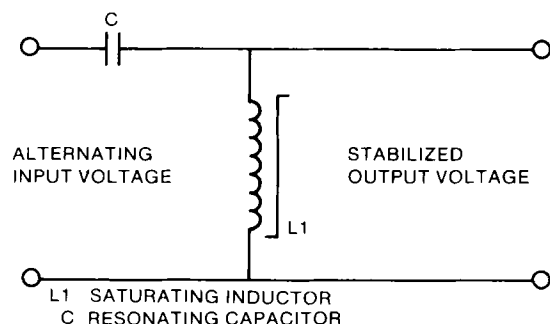
Fig 1 Basic Series Ferroresonant Voltage Regulator
