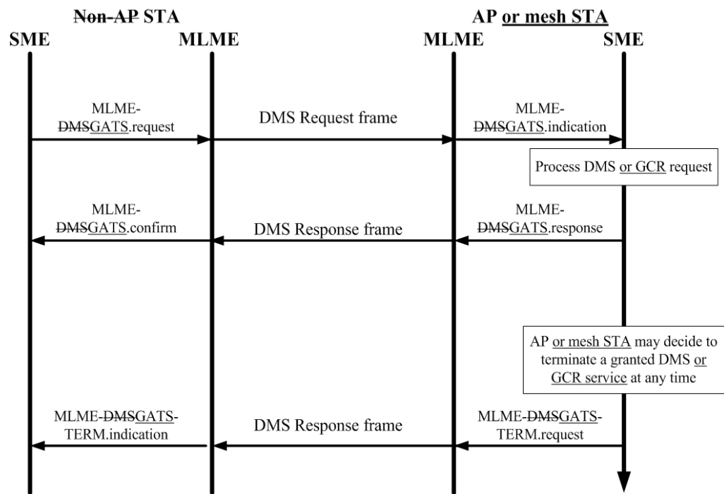
Figure 6-25—DMS or GCR setup protocol exchange
