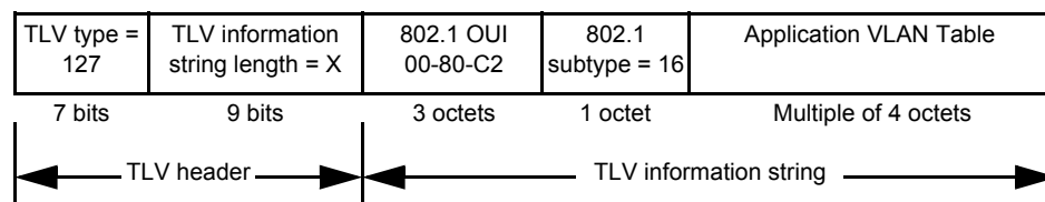
Figure D-15—Application VLAN TLV format
