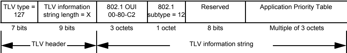
Figure D-12—Application Priority TLV format
