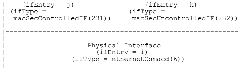
i, j, k are ifIndex to indicate an interface stack in the ifTable. Figure : PAC Interface Stack
