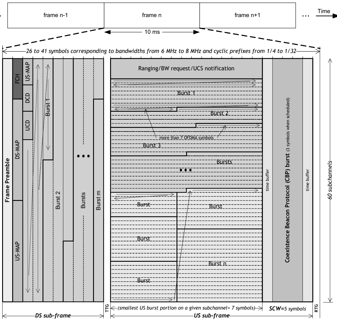
Figure 13 — Example of a time/frequency structure of a MAC frame
