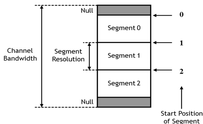
Figure 13f—Segment structure
