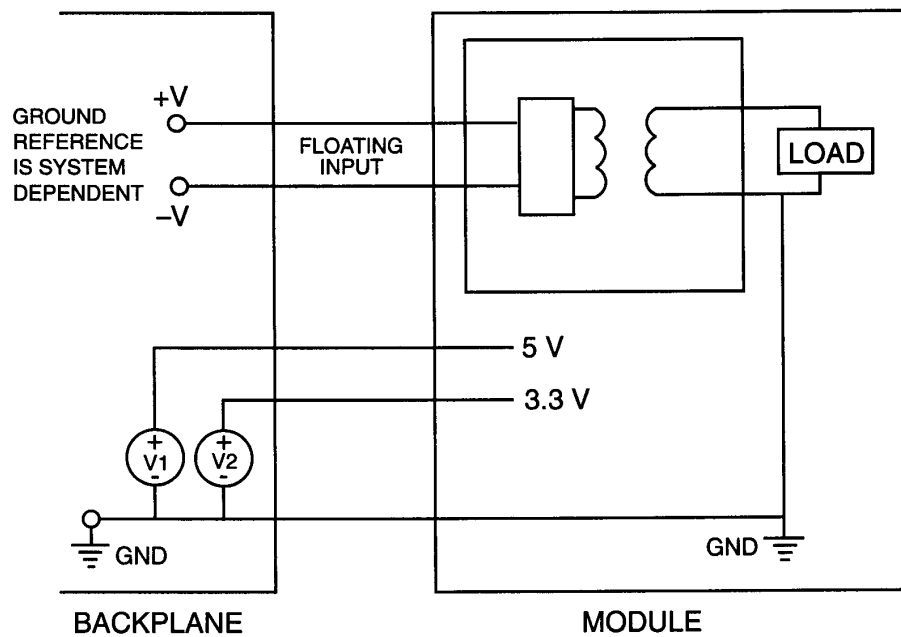
Figure 4-1—Digital power rails
