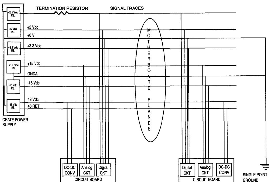
Figure 4-3—Example of logic & analog power & ground configuration
