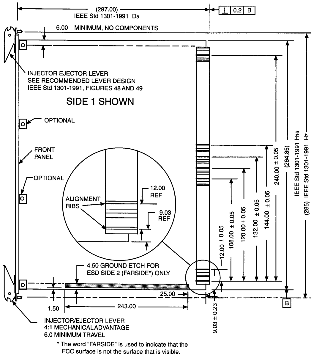
Figure 4-4—View of plug-in module
