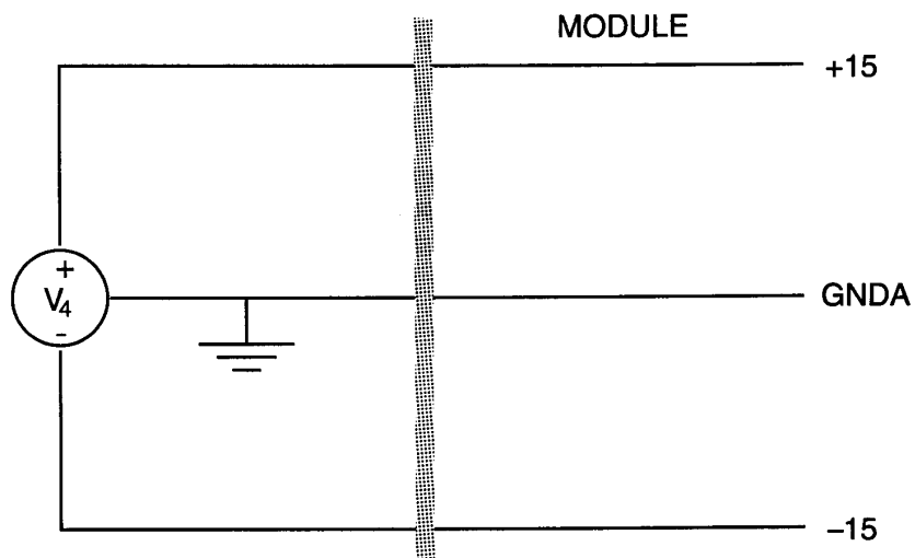
Figure 4-2—Analog power rails
