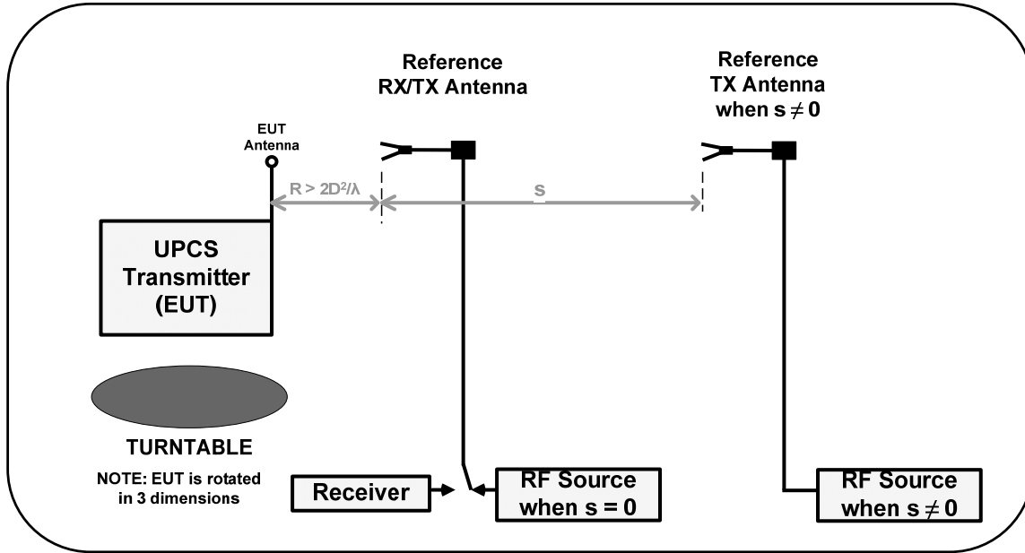
Figure 2—Radiated measurements in free-space environment
