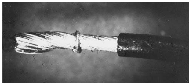
Figure 4-8 Illustration of Partially Solderable Stranded Wire Showing Incomplete Fillet
