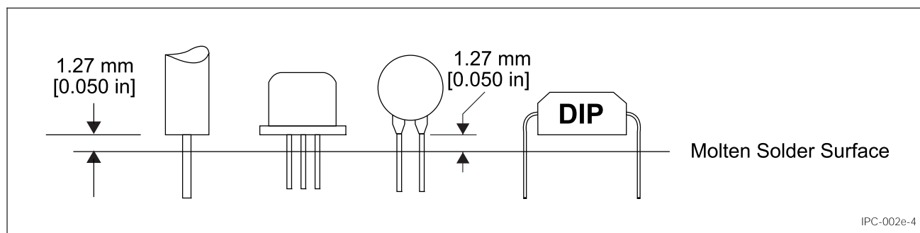
Figure 4-3 Solder Dipping Depth for Through-Hole Components
