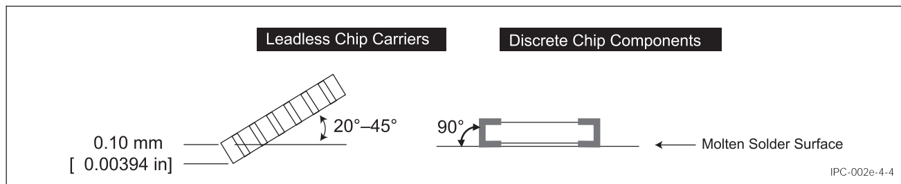
Figure 4-4 Leadless Component Immersion Depth
