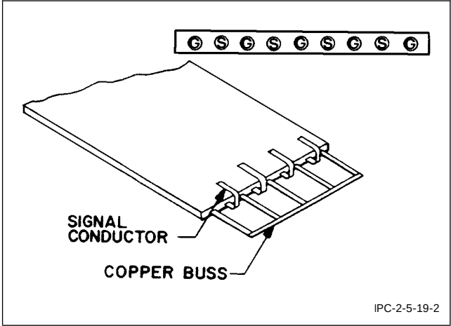
Figure 3 Cable Preparation
