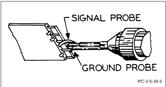
Figure 4 Cable Connection
