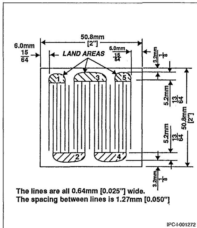
Figure 1 Insulation resistance test pattern
