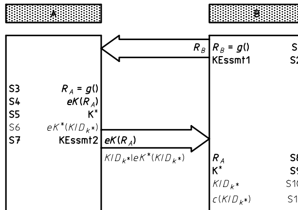
Figure 2 — Key Exchange symmetric symmetric mutual timeliness
