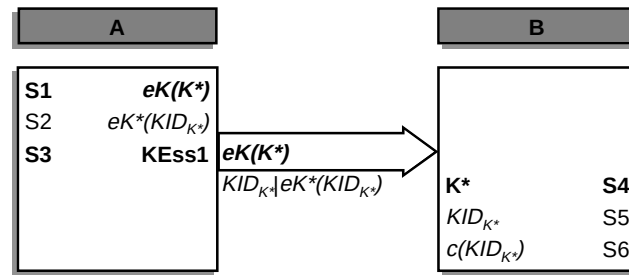
Figure 1 — Key Exchange symmetric symmetric
