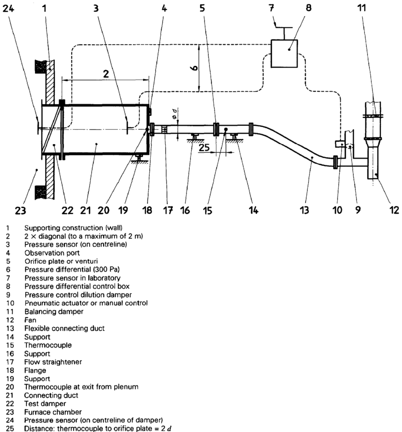
Figure 1 — Example of general test arrangement
