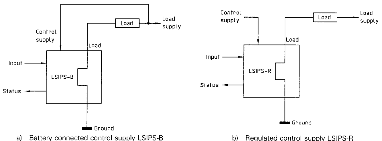
Figure 1 — Control supply
