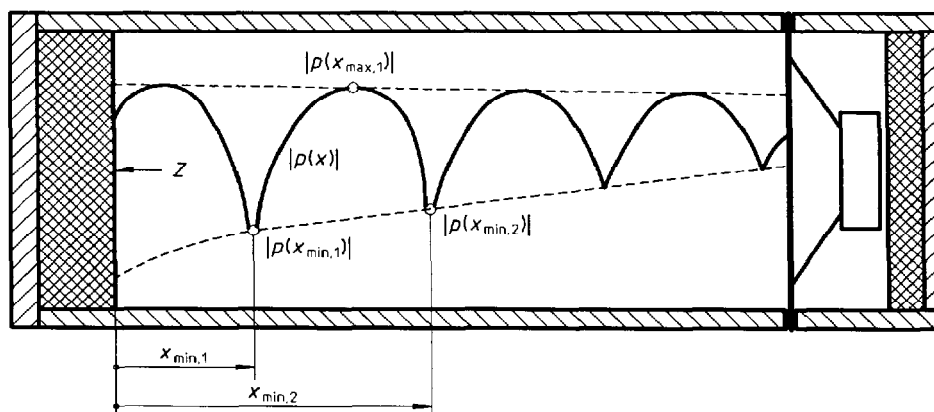
Figure 1 — Standing wave pattern in a test tube
