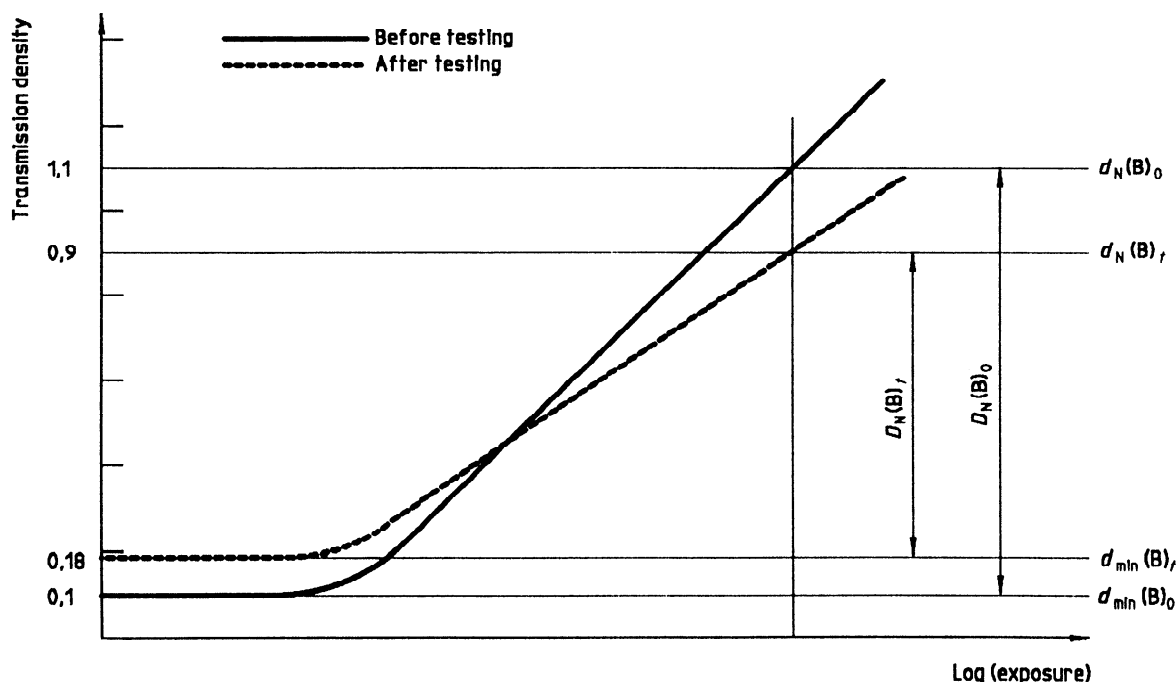
Figure 1 — Blue transmission density of a neutral patch of a transparency-type colour material
