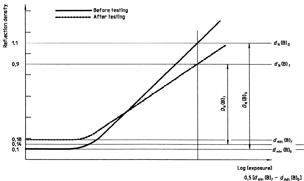
Figure 2 — Blue reflection density of a neutral patch of a reflection-type colour material
