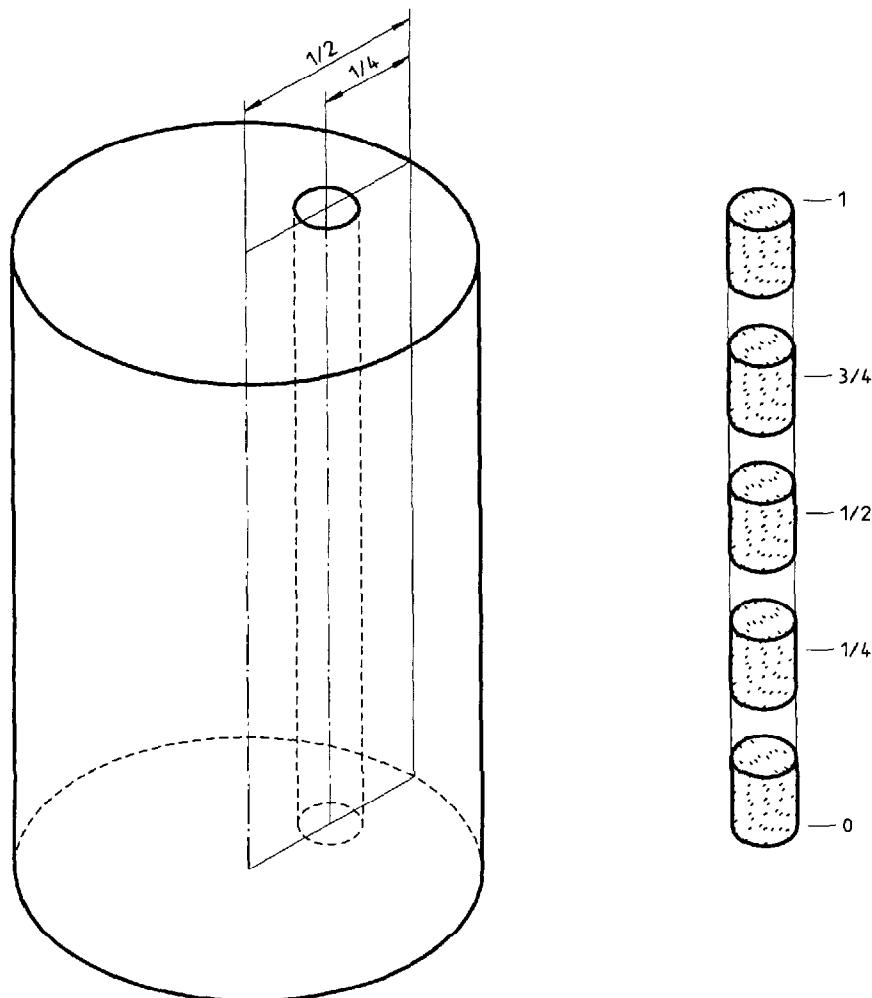
Figure 2 — Sampling of homogeneous waste forms
