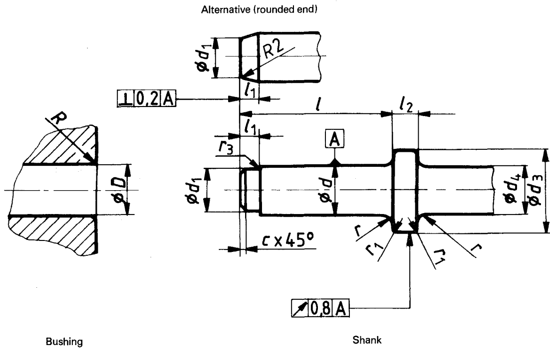
Figure 1 — Coal pick shanks and corresponding chuck bushings
