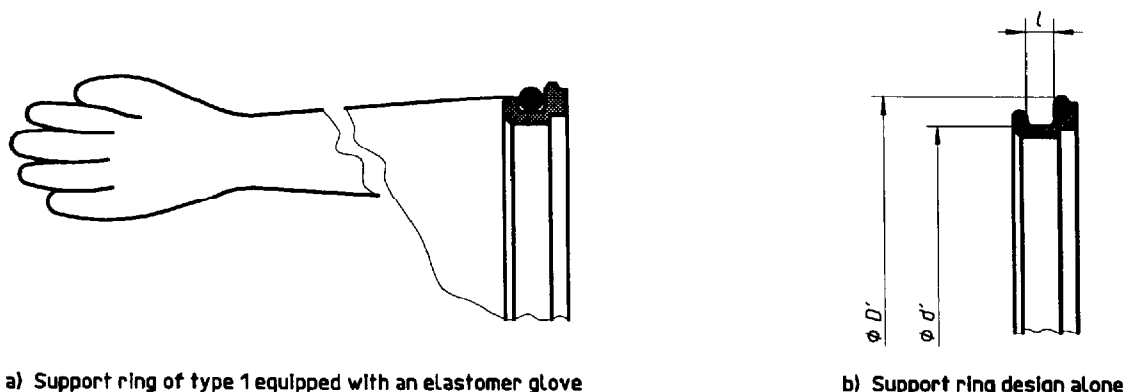
Figure 8 — Elastomeric glove fitted on an ejectable support ring of type 1
