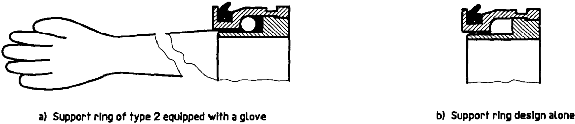
Figure 9 — Elastomeric glove fitted on an ejectable support ring of type 2
