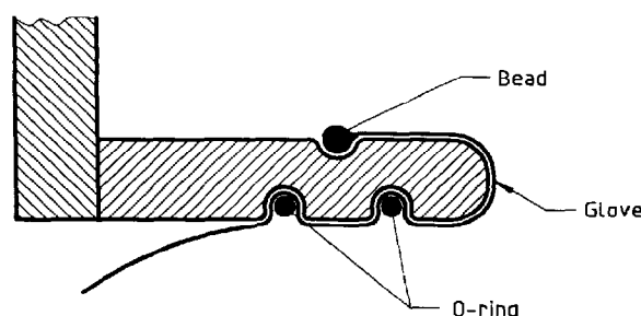
Figure 5 — Method of glove attachment on ports having one external groove and two internal grooves
