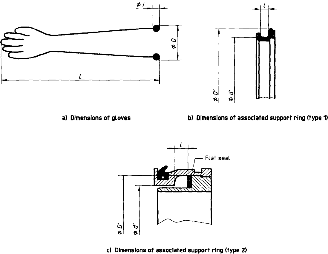
Figure 10 — Dimensions of gloves fitted on ejectable support rings
