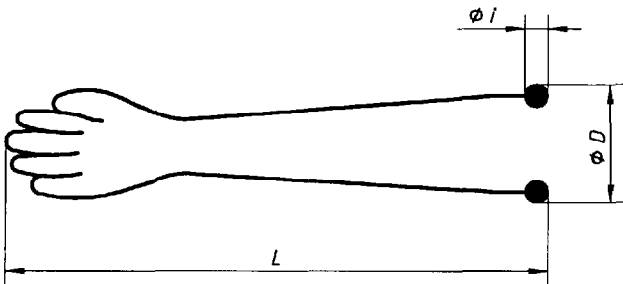
Figure 6 — Glove for glove ports
