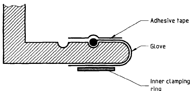
Figure 2 — First alternative method of glove attachment to glove ports having two external grooves
