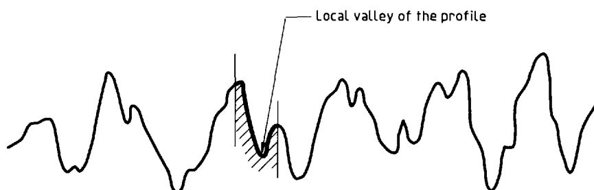
Figure 2 — Local valley of profile
