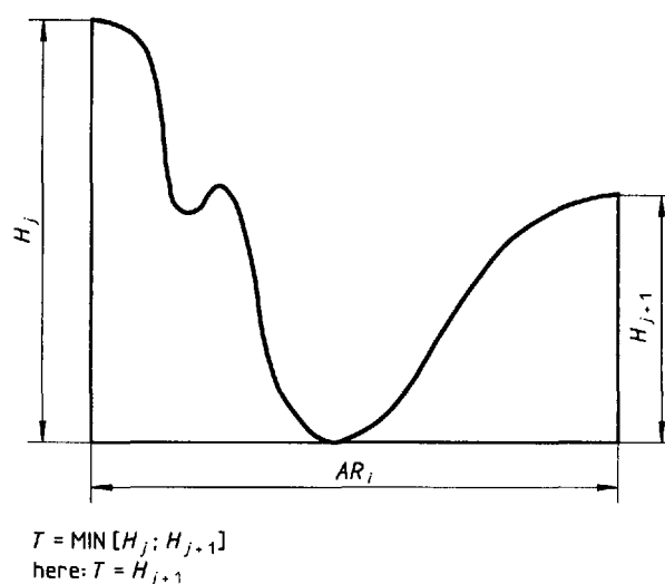
Figure 3 — Roughness motif
