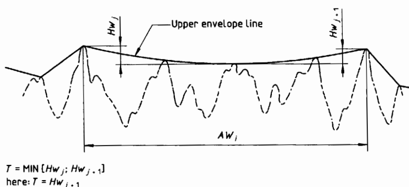
Figure 5 — Waviness motif
