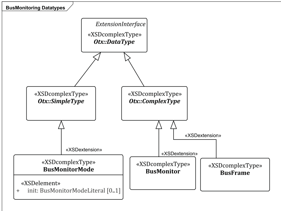
Figure 10 — BusMonitoring - Datatypes
