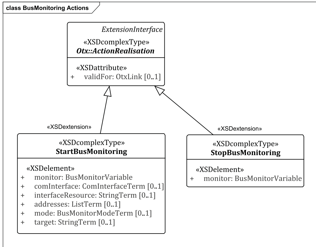
Figure 14 — BusMonitoring – Actions
