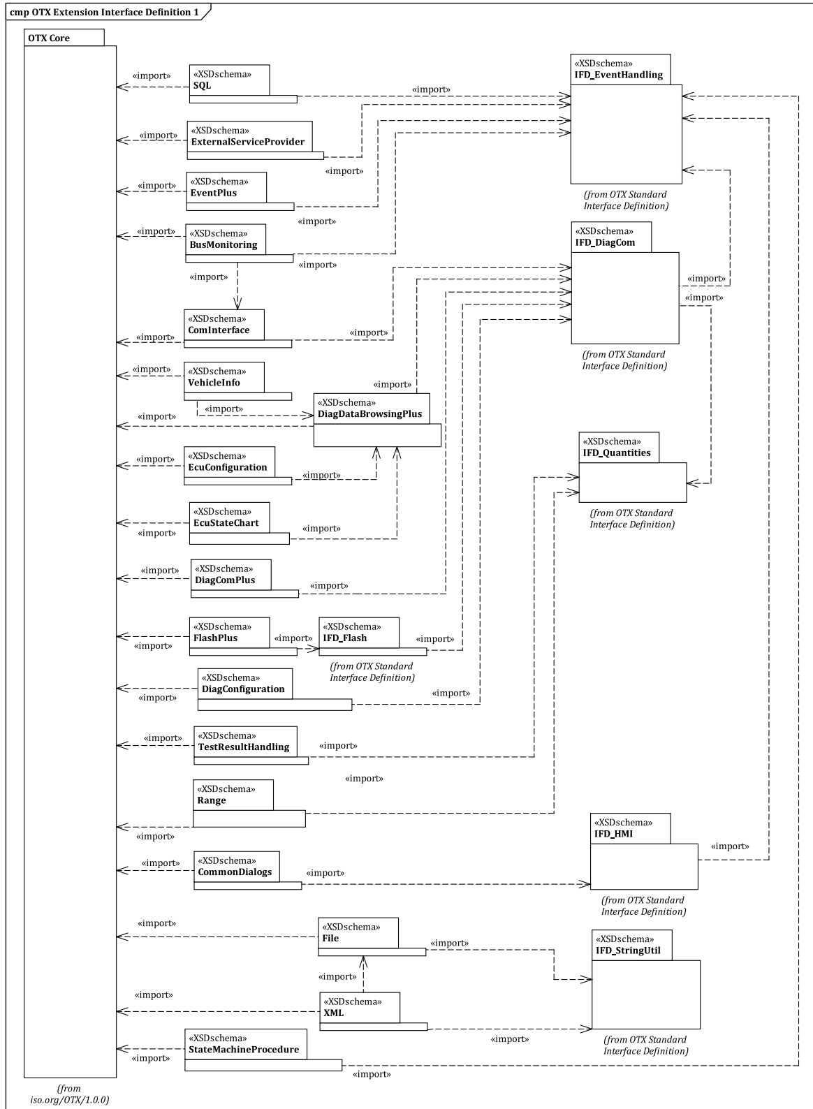
Figure 3 — Overview OTX schema dependencies 1
