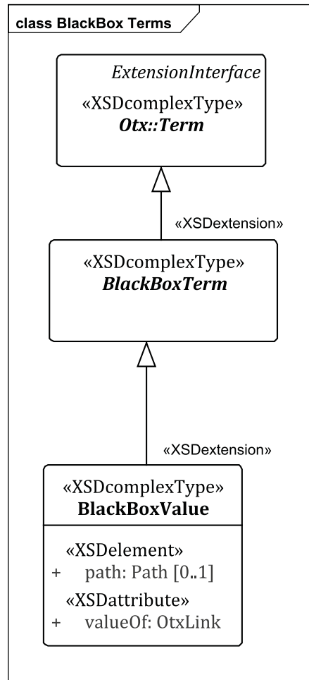
Figure 9 — BlackBox – Terms
