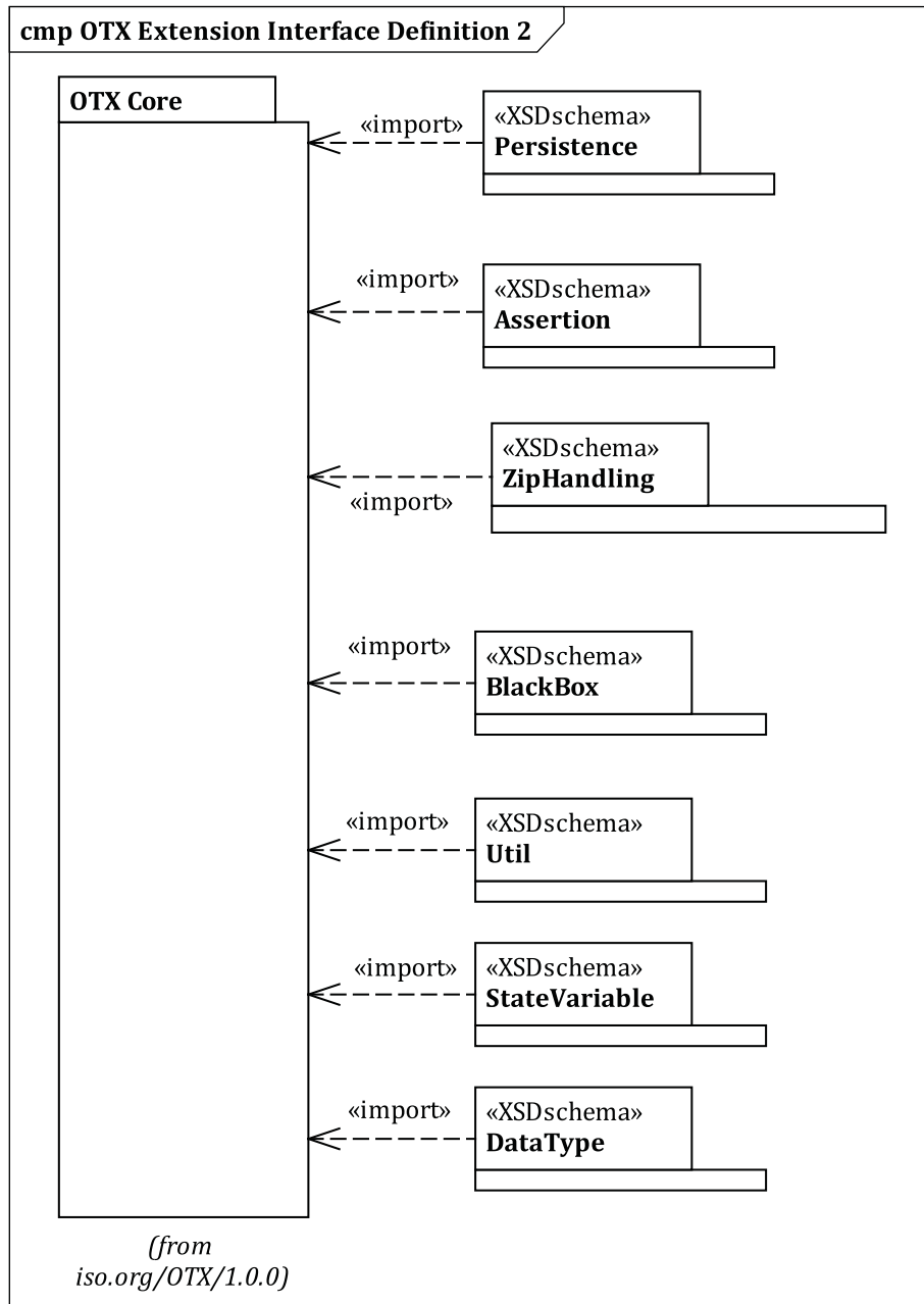
Figure 4 — Overview OTX schema dependencies 2
