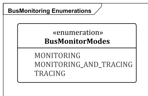
Figure 11 — BusMonitoring – Enumerations
