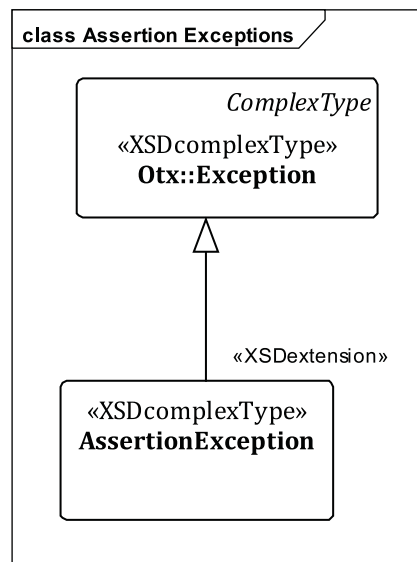
Figure 5 — Assertion – Exceptions
