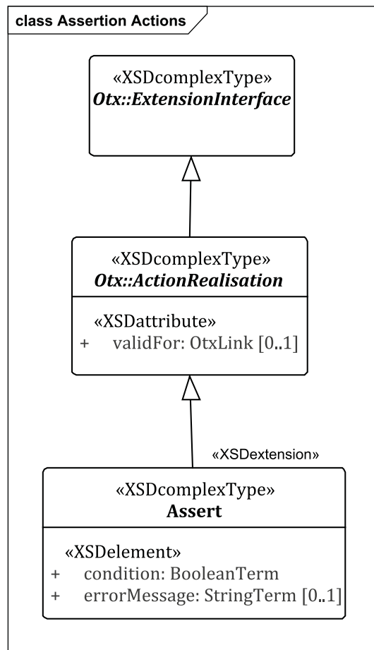
Figure 6 — Assertion – Actions
