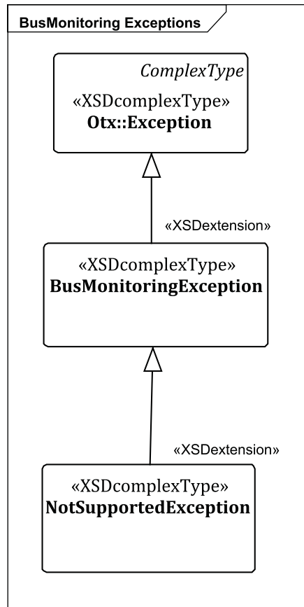
Figure 12 — BusMonitoring – Exceptions
