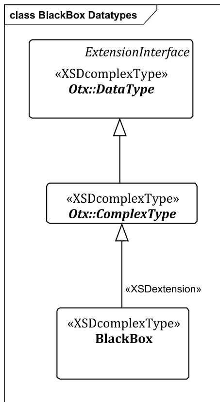
Figure 7 — BlackBox – Datatypes
