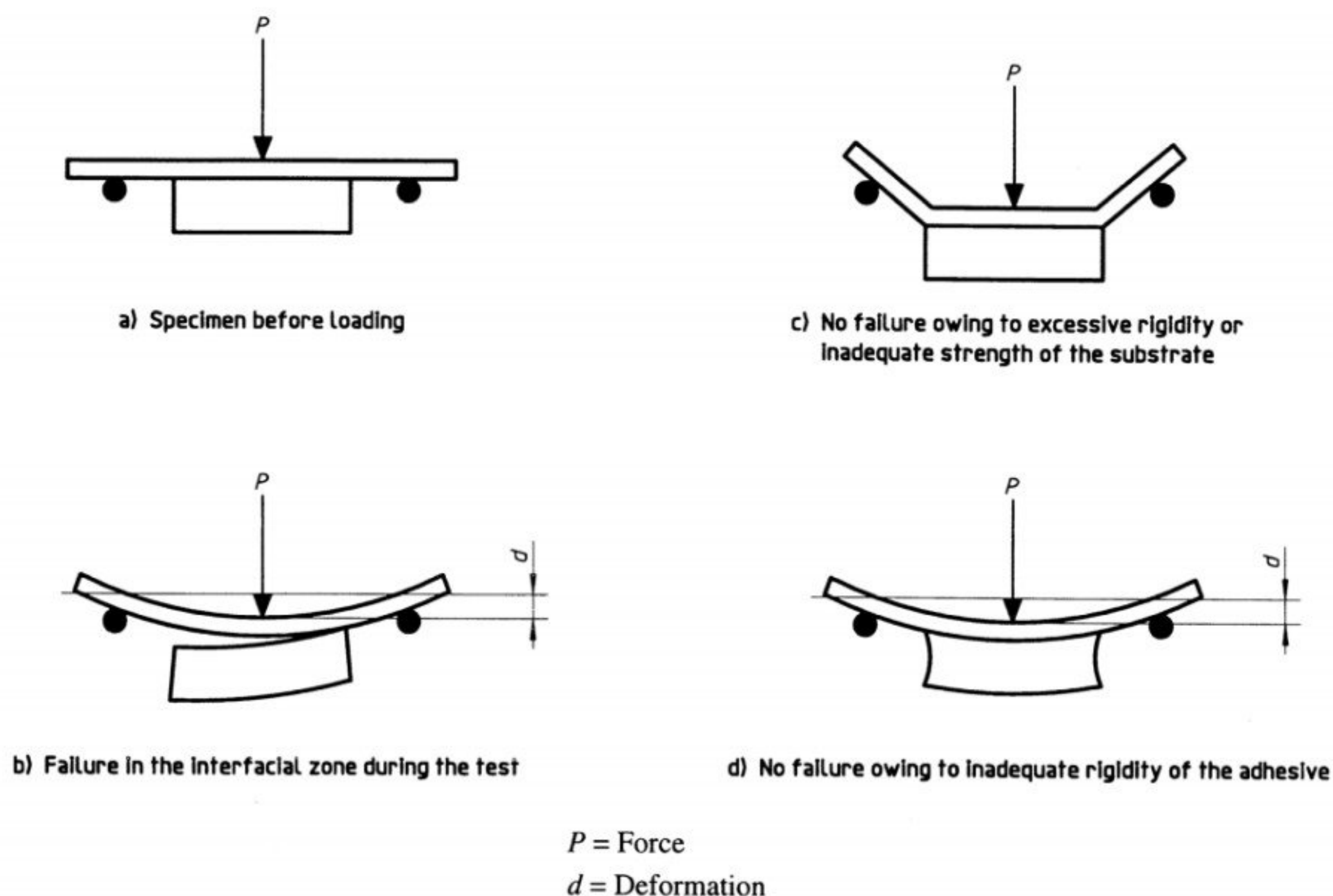
Figure 2 — Principle of the test
