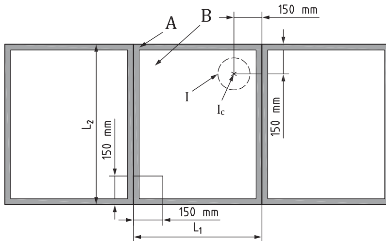
b) Specimen 2: impact area of wood lumber missile impact test for windows (incl. skylights), doors or curtain walling intended to be installed combined together and tested by joining at least three lites into one mounting frame
