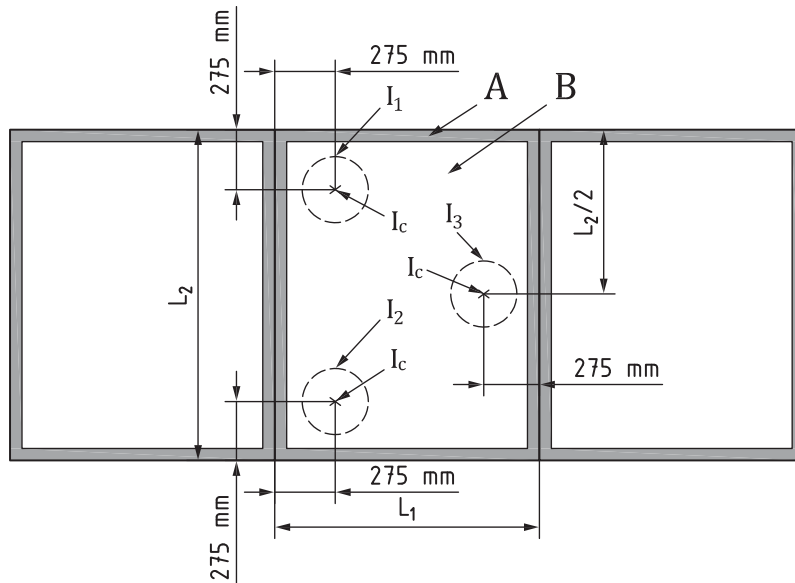
a) Specimen 1: impact area of steel ball impact test for windows (incl. skylights), doors or curtain walling intended to be installed combined together and tested by joining at least three lites into one mounting frame
