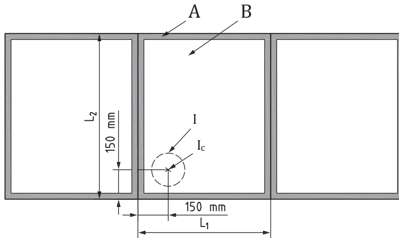
b) Specimen 2: impact area of wood lumber missile impact test for windows (incl. skylights), doors or curtain walling intended to be installed combined together and tested by joining at least three lites into one mounting frame
