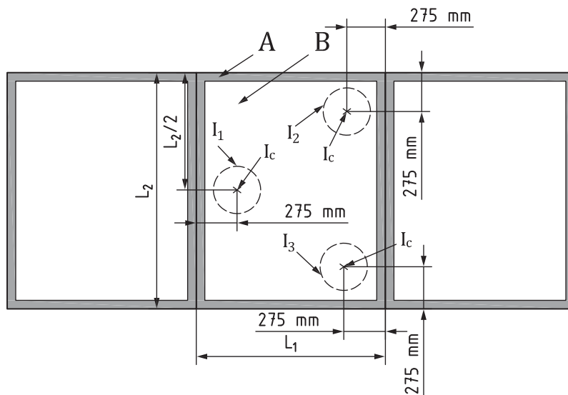
a) Specimen 1: impact area of steel ball impact test for windows (incl. skylights), doors or curtain walling intended to be installed combined together and tested by joining at least three lites into one mounting frame
