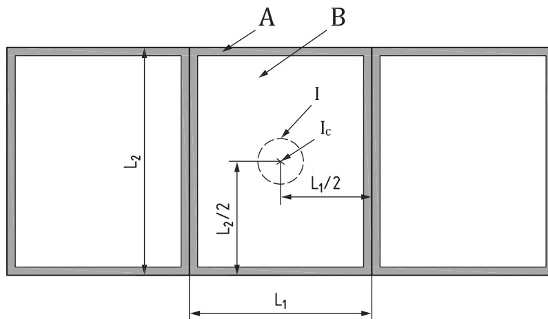
a) Specimen 1: impact area of wood lumber missile impact test for windows (incl. skylights), doors or curtain walling intended to be installed combined together and tested by joining at least three lites into one mounting frame
