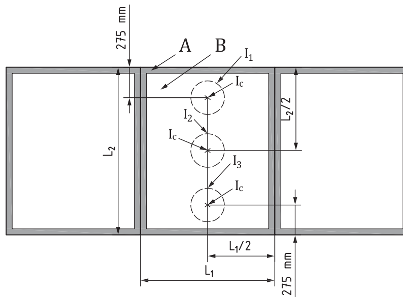
c) Specimen 3: impact area of steel ball impact test for windows (incl. skylights), doors or curtain walling intended to be installed combined together and tested by joining at least three lites into one mounting frame
