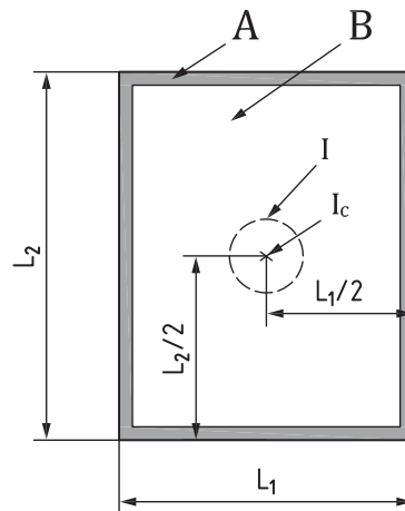
a) Specimen 1: impact area of wood lumber missile impact test for individual windows (incl. skylights), doors or curtain walling tested separately
