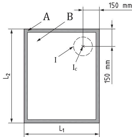
c) Specimen 3: impact area of wood lumber missile impact test for individual windows (incl. skylights), doors or curtain walling tested separately
