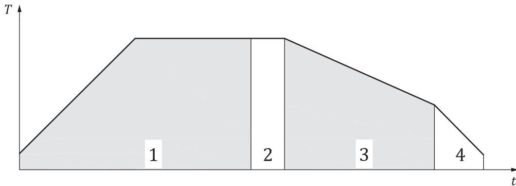
Figure 4 — Typical temperature profile for thermoset matrices
