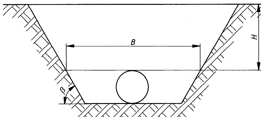
Figure 4 — Trench with sloping walls
