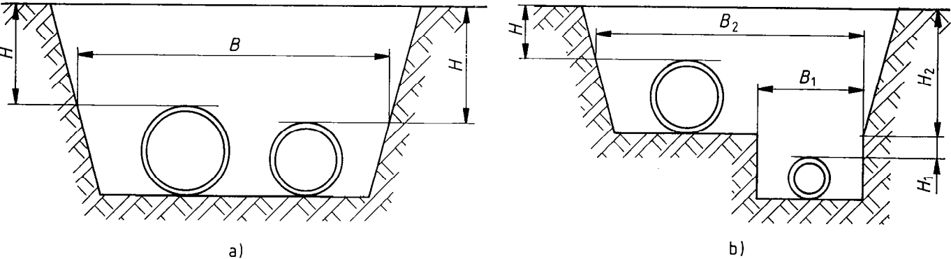
Figure 3 — Type 3 of pipe-laying
