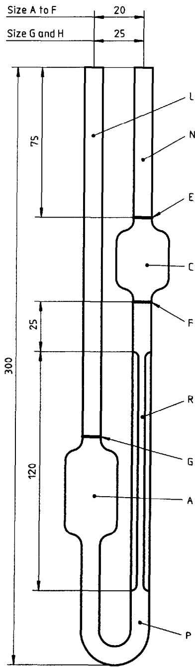
Figure A.3 — BS/U-tube viscometer
