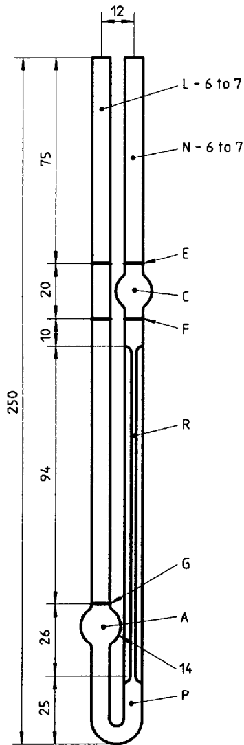
Figure A.4 — BS/U/M miniature viscometer
