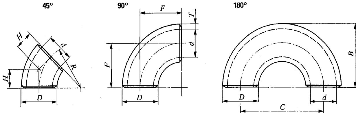
Figure 2 – Bends 3D
