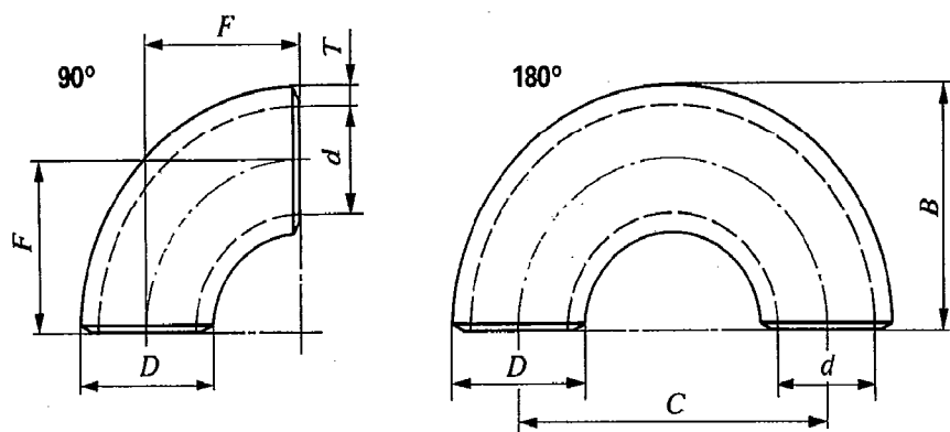
Figure 1 — Bends 2D
