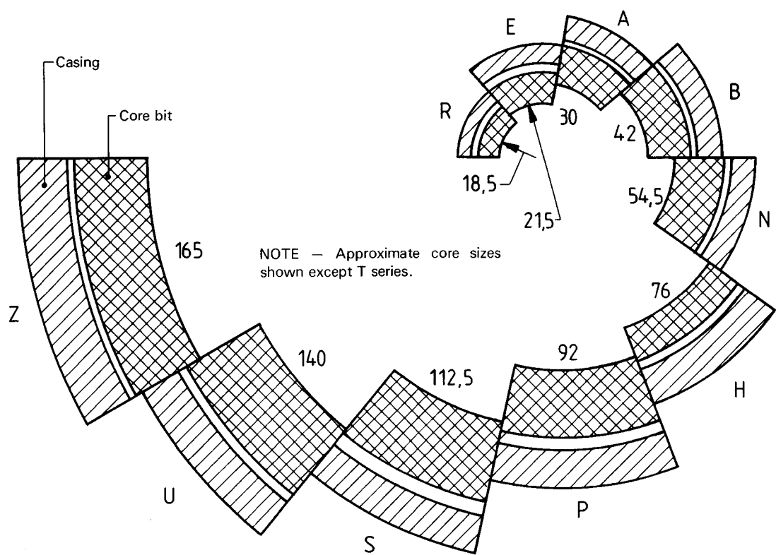
Figure 5 — General relation of casing to core bit
