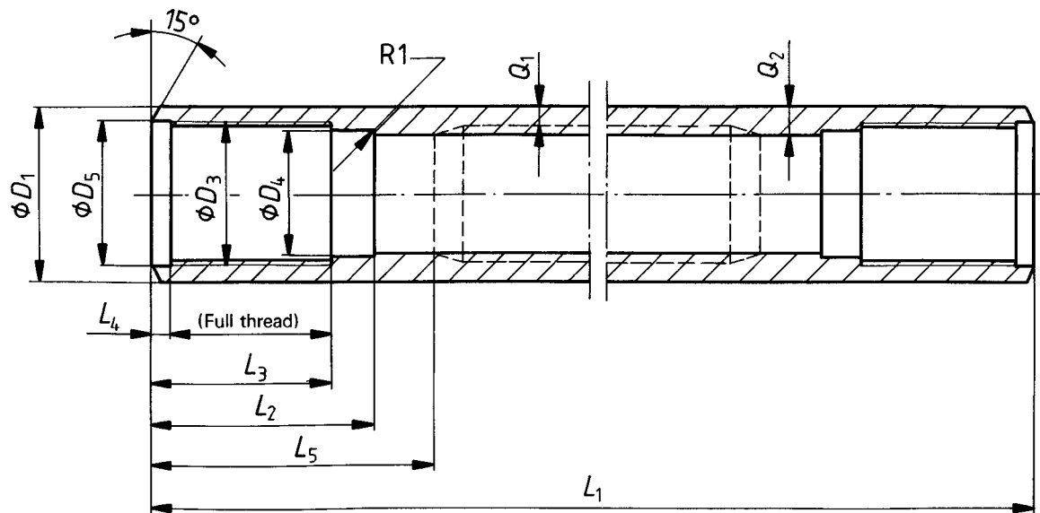
Figure 6 — Fishing rod (see table 10)
