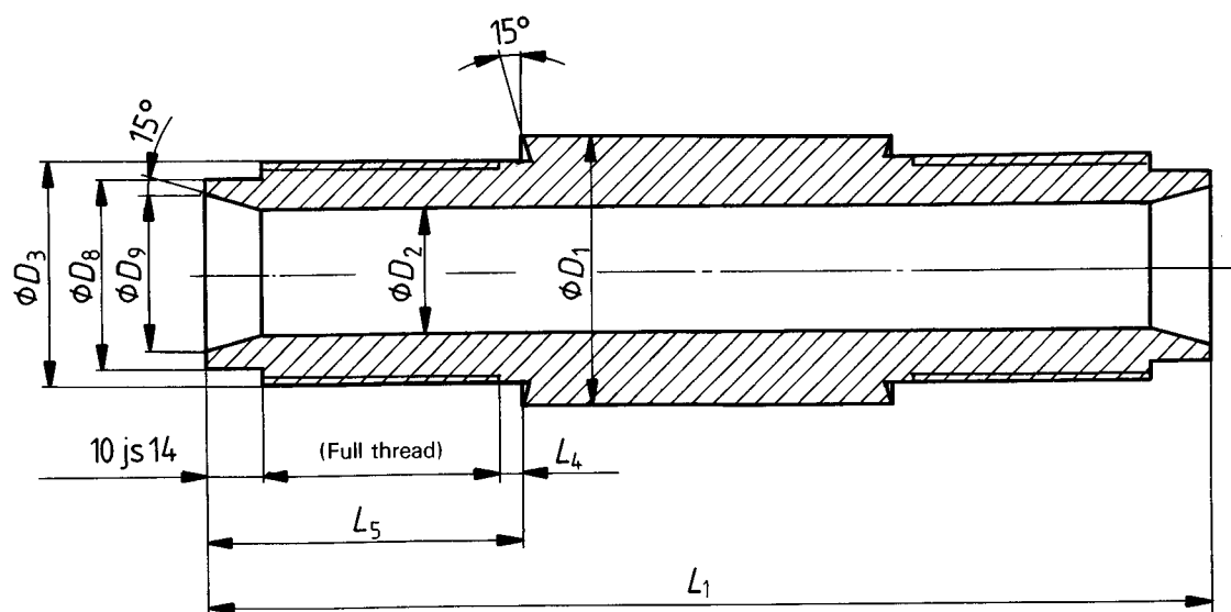
Figure 7 — Fishing-rod coupling (see table 11)
