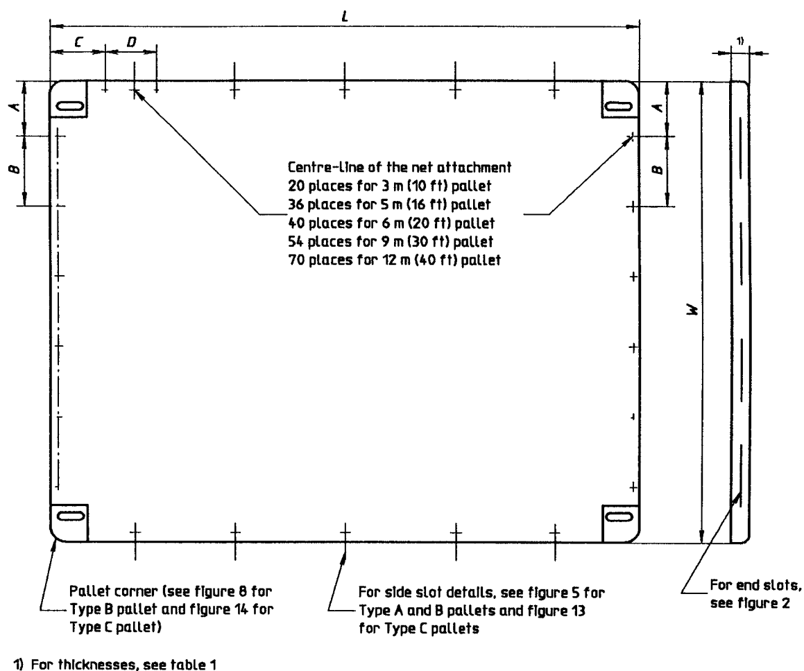
Figure 1 — Pallet dimensions
