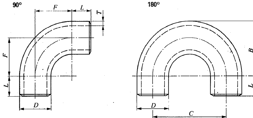
Figure 2 — Bends 3D with straight ends
