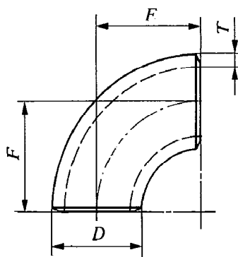
Figure 3 — Bends 5D
