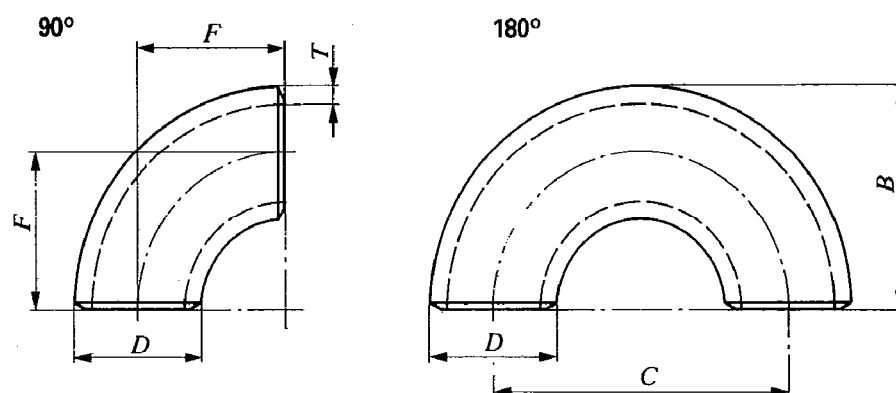
Figure 1 — Bends 3D without straight ends
