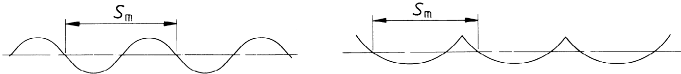
Figure 4 — Type B2 grooves (insensitive grid)
