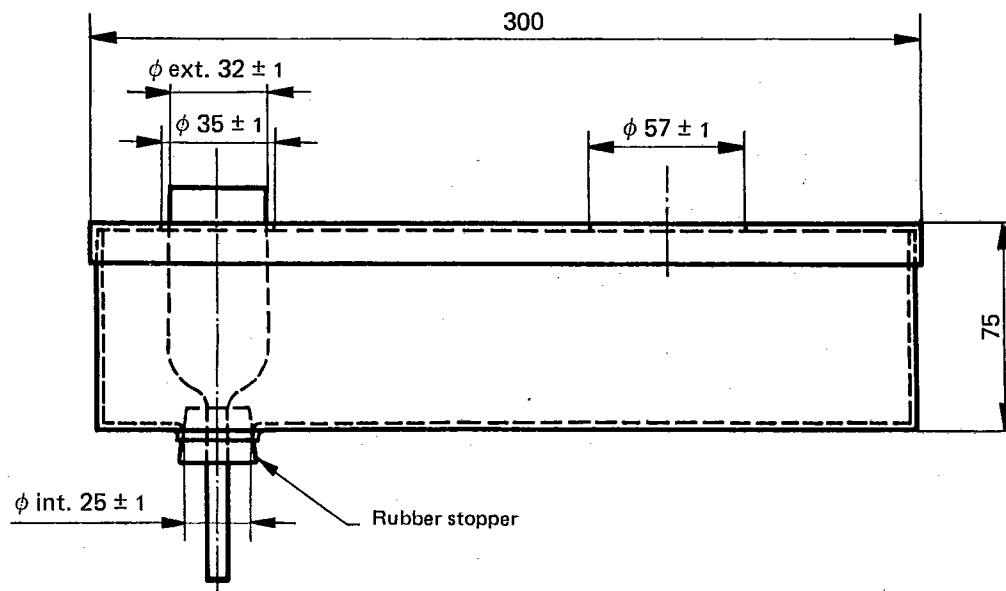
FIGURE 2 — Hot water bath for determination of matter insoluble in hot alcohol (method I)
