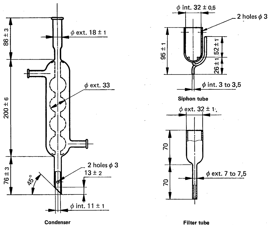
FIGURE 1 — Extraction apparatus for determination of matter insoluble in hot alcohol (method I)
