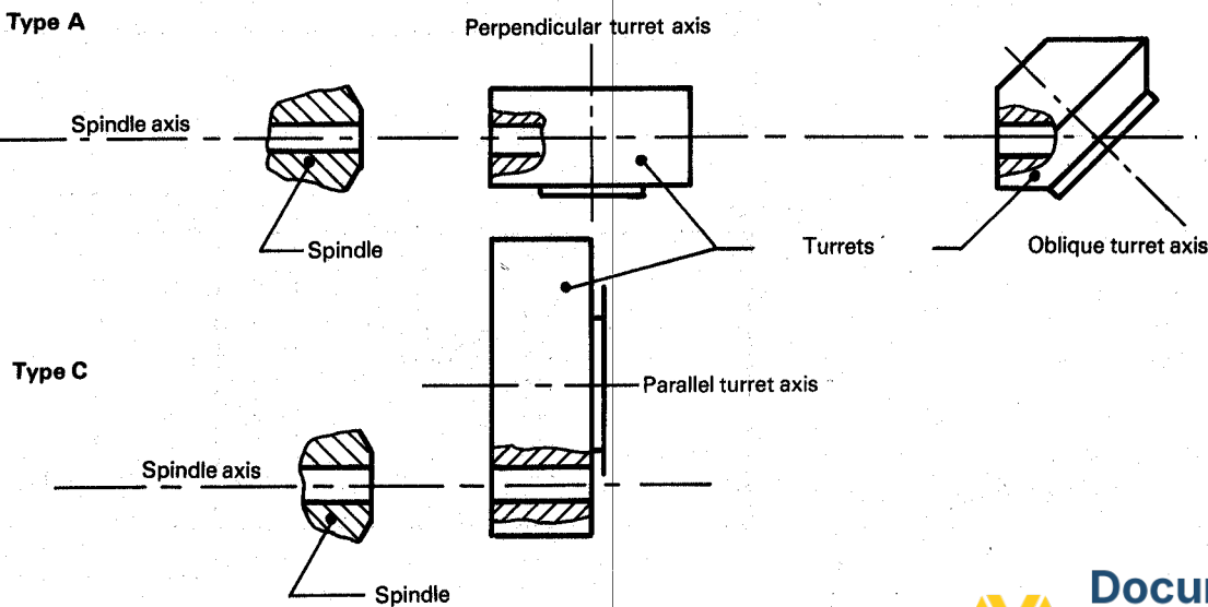
Different types of capstan turret
