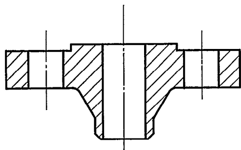
Type 11 Welding neck flange
