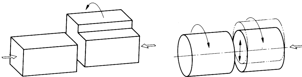
Figure 15 — Orbital friction welding Figure 15 — Soudage par friction orbitale
