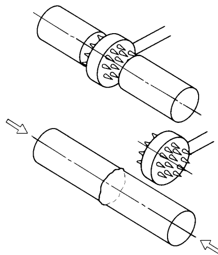
b) Opened assembly b) Joint ouvert
