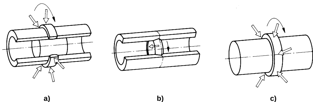
Figure 16 — Radial friction welding Figure 16 — Soudage par friction radiale
