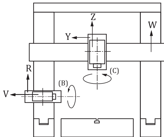
a) One vertical spindle head mounted on the cross-rail and one horizontal spindle head mounted on the left-hand column
