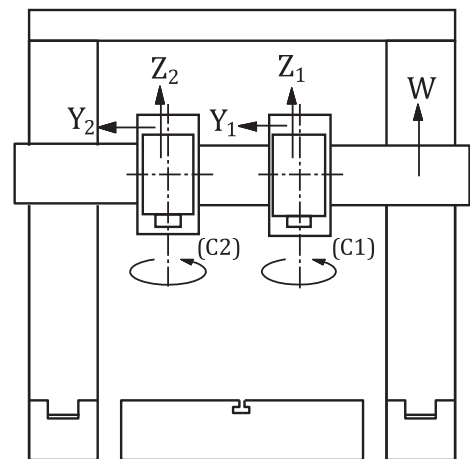
b) Two vertical spindle heads mounted on the cross-rail
