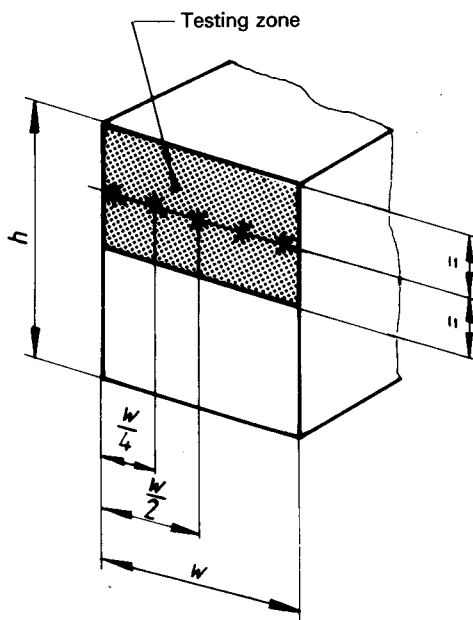
Figure 2 — Hardness testing
