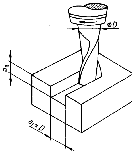
Figure 1 — Slot milling
