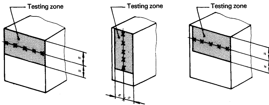
Figure 4 — Hardness testing
