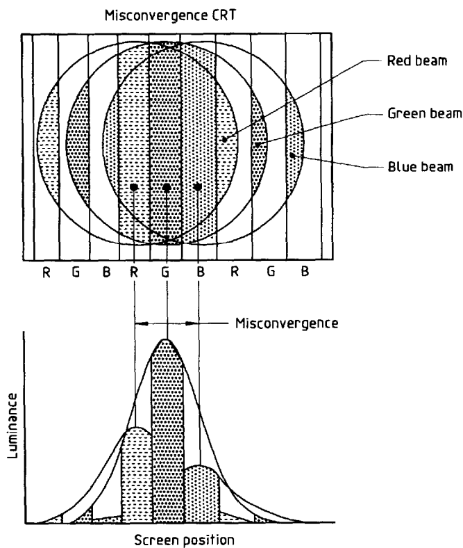
Figure 4 – CRT misconverged R,G,B electron beams
