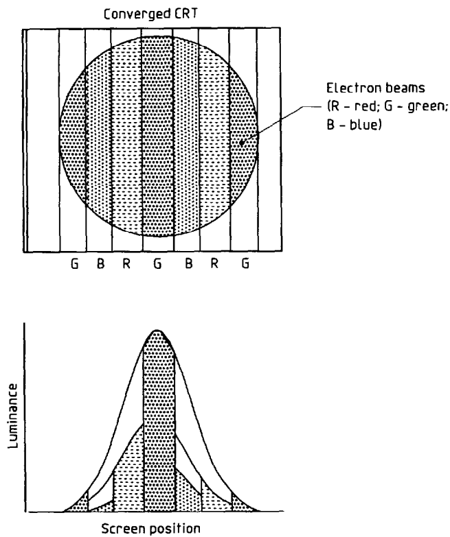
Figure 3 – CRT converged R,G,B electron beams
