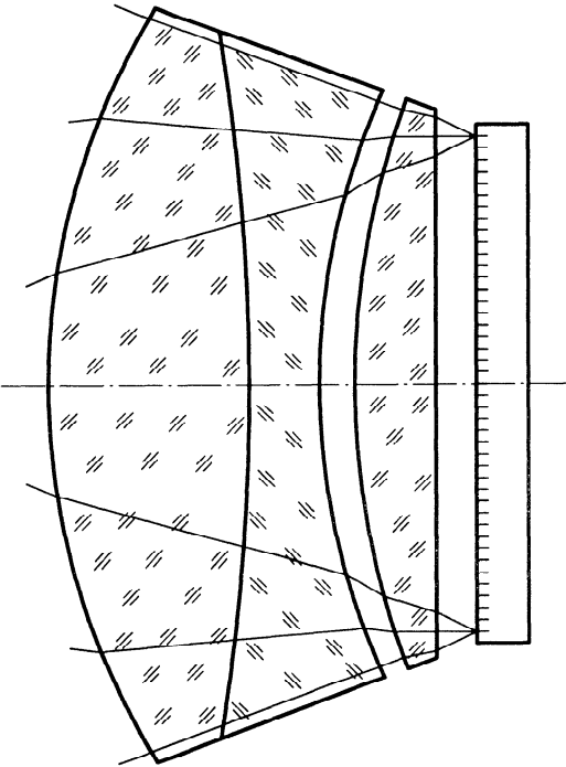
Figure 1 — Mirror half lens
