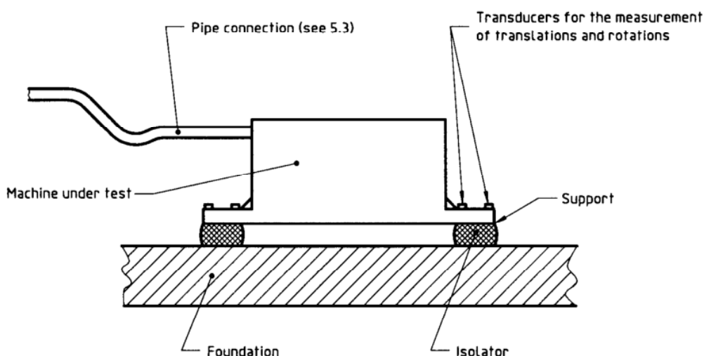
Figure 1 — Test arrangement
