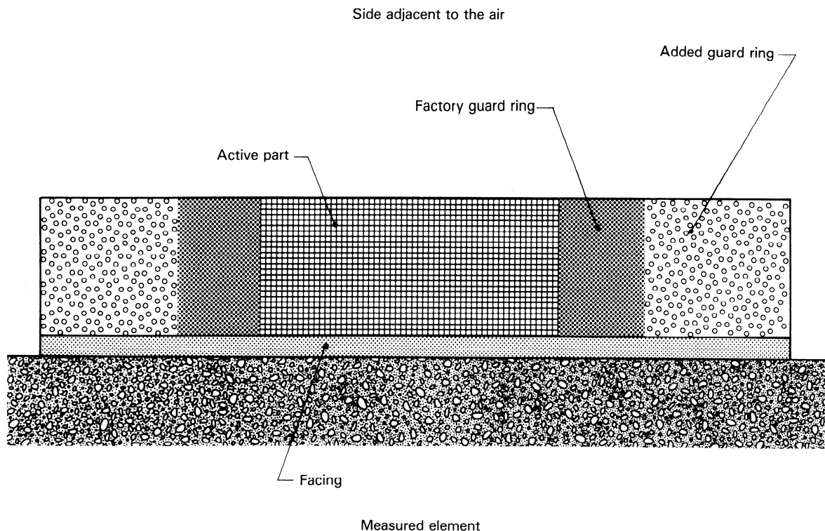
Figure 1 — Section through a typical heat flowmeter showing the various parts (the vertical scale is enlarged)
