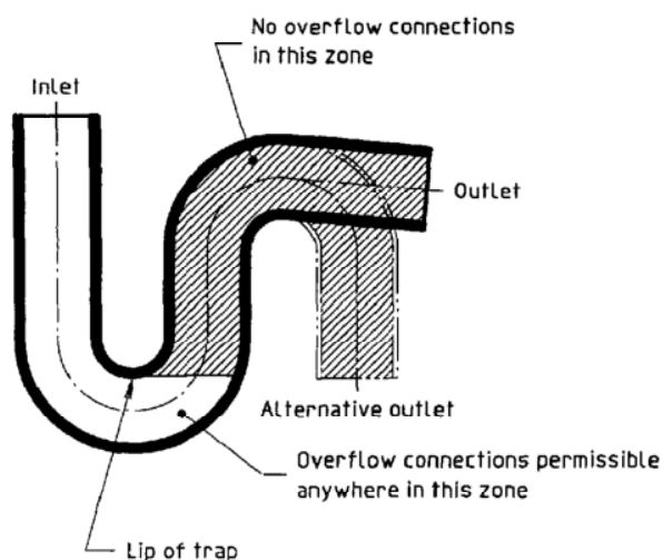
Figure 6 — Positions of inlets and outlets
