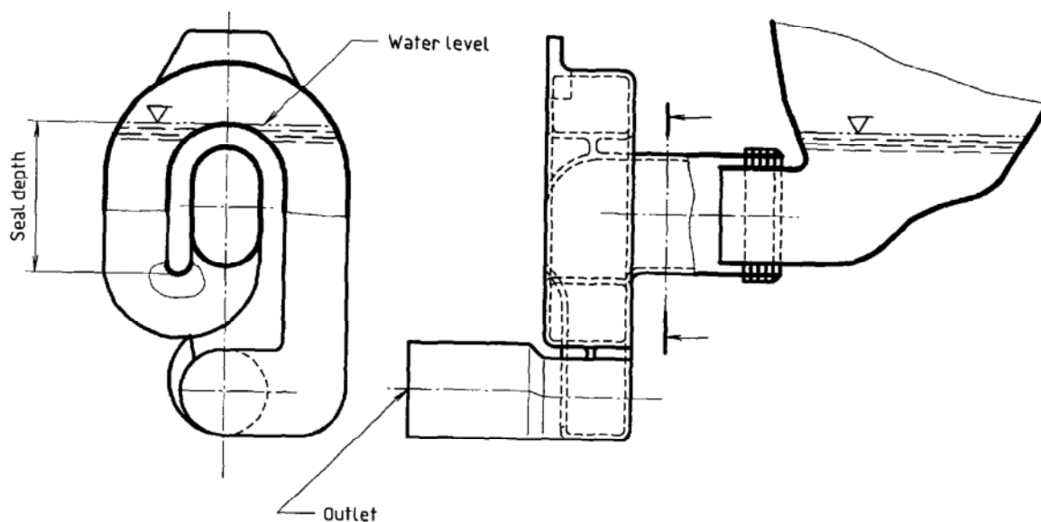
Figure 4 — Urinal trap
