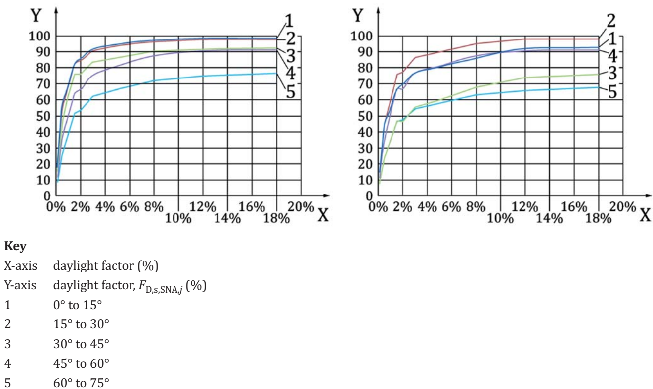
Figure A.11 — Example of a set of functions used to determine the daylight supply factor F_{D,s,SN\alpha,j} and F_{D,s,SA,j} as a function of D and \gamma according to Table A.7 for \bar{E}_m = 500 lx and a south-facing facade
