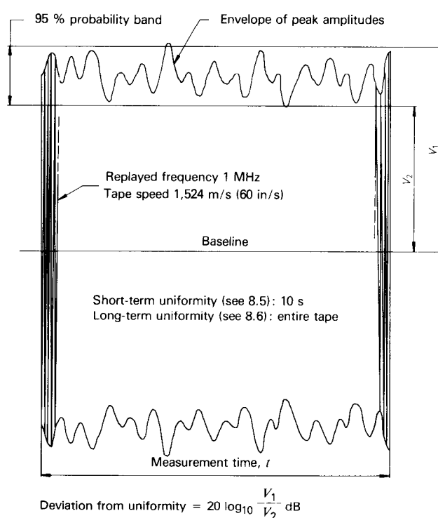
Figure 1 — Replayed waveform for output uniformity test
