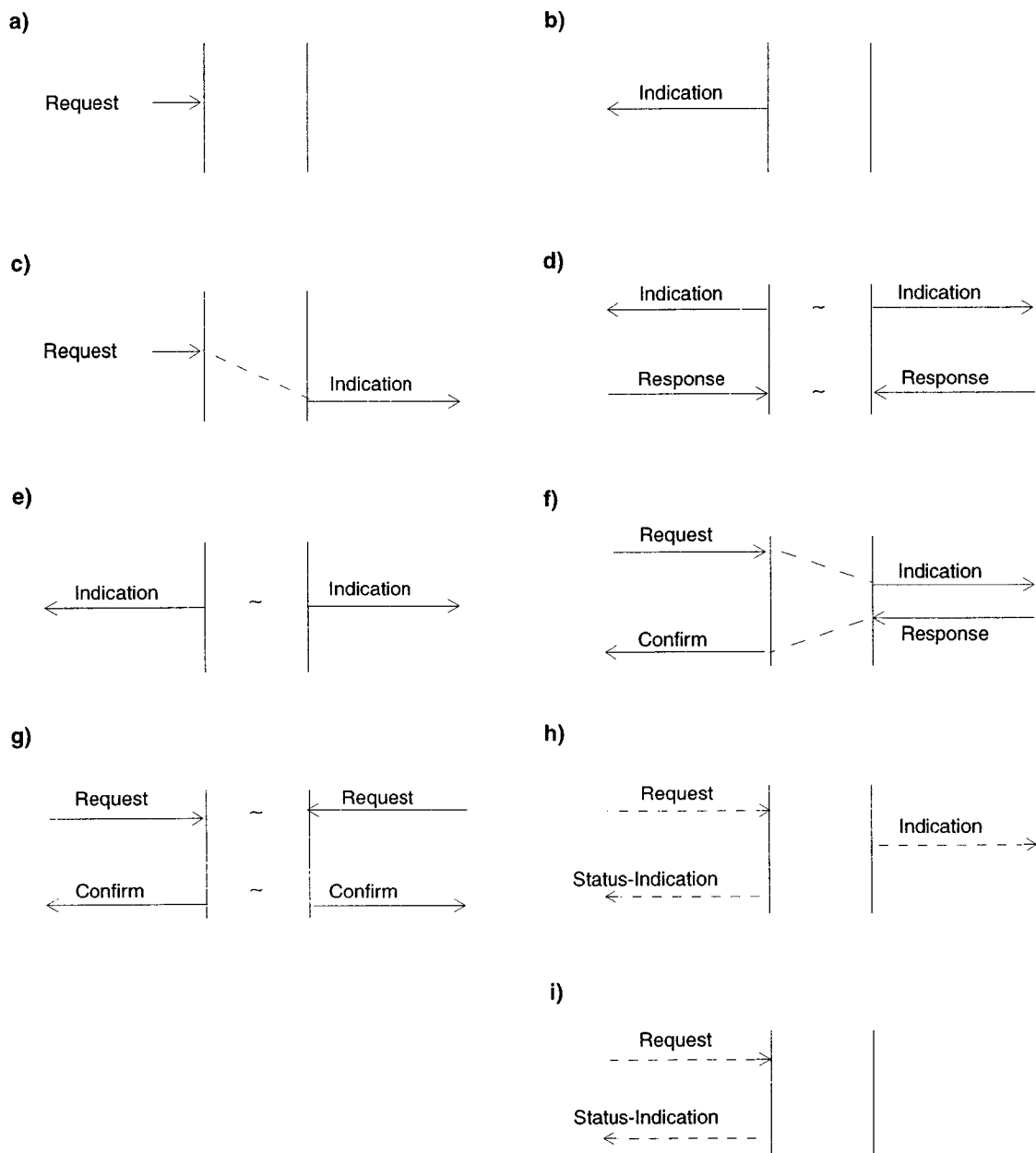
Figure 3—Time-sequence diagrams
