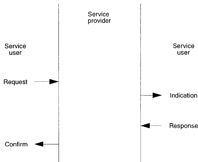
Figure 2—Service primitives
