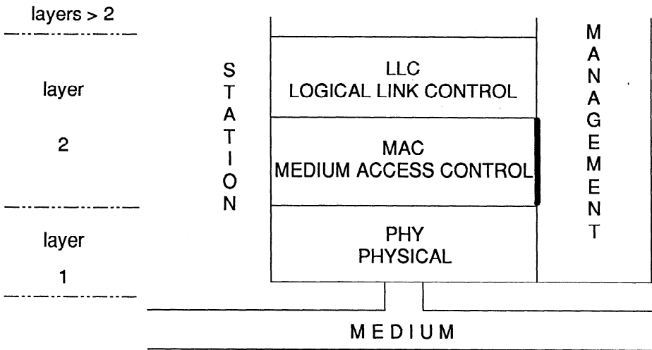
Fig 3-1 Relation to LAN Model
