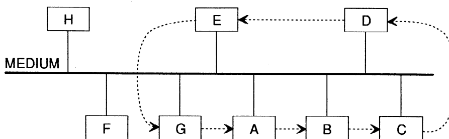
Fig 1-2 Logical Ring on Physical Bus
